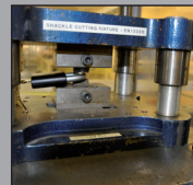
Shackle cutting
